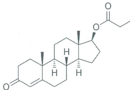
Testosterone propanoate
