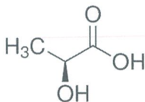
Lactic acid
