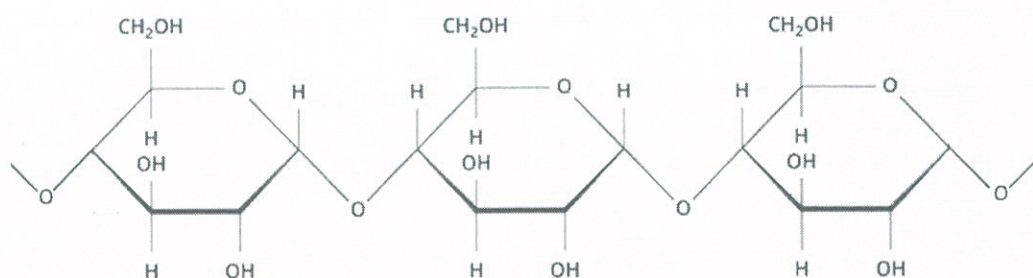
Starch
