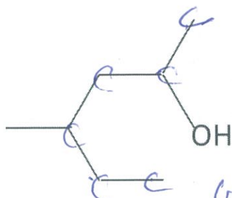
Compound A
