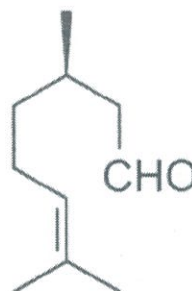
C – citronellal
