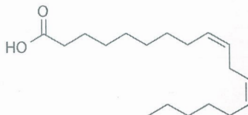
Linoleic Acid
