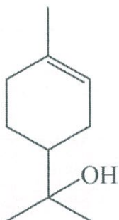
A – terpineol
